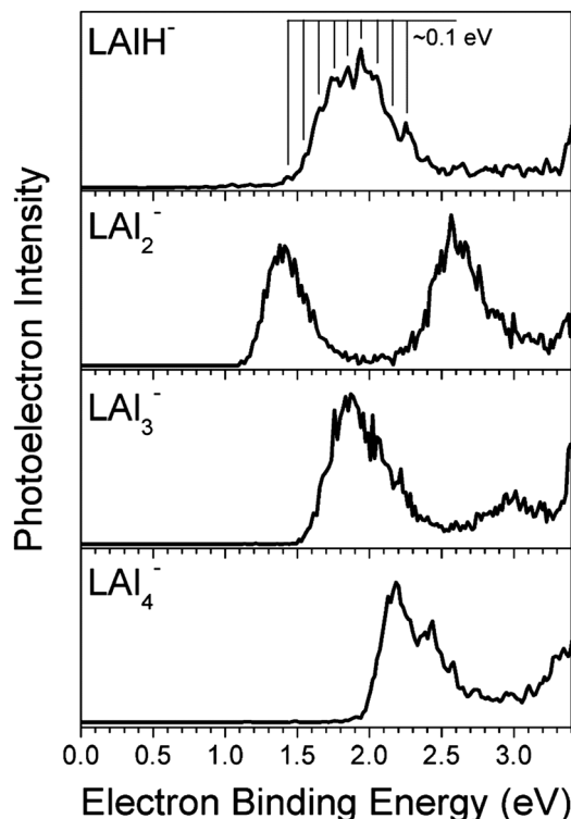
Fig. 2 Photoelectron spectra of \text{LAIH}^- , \text{LAI}_2^- , \text{LAI}_3^- and \text{LAI}_4^- anions recorded with 3.49 eV photons ( \text{L} = \text{N}[\text{Si}(\text{Me})_3]_2 ).
