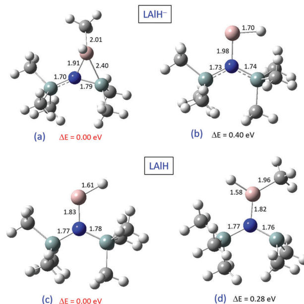
Fig. 3 Calculated structures of \text{LAIH}^{-/0} isomers. Also shown are their relative energies in eV ( \text{L} = \text{N}[\text{Si}(\text{Me})_3]_2 ).
